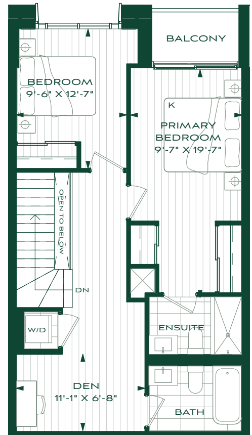
FLOOR 2
